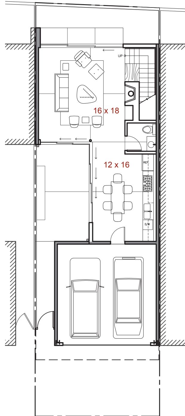
1ST FLOOR 582.90 SF GARAGE 334.56 SF
