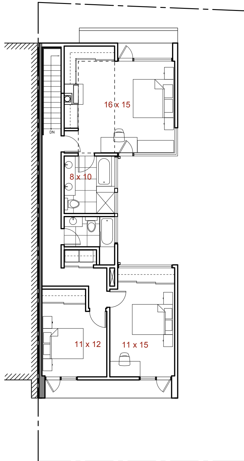
2ND FLOOR 956.81 SF
